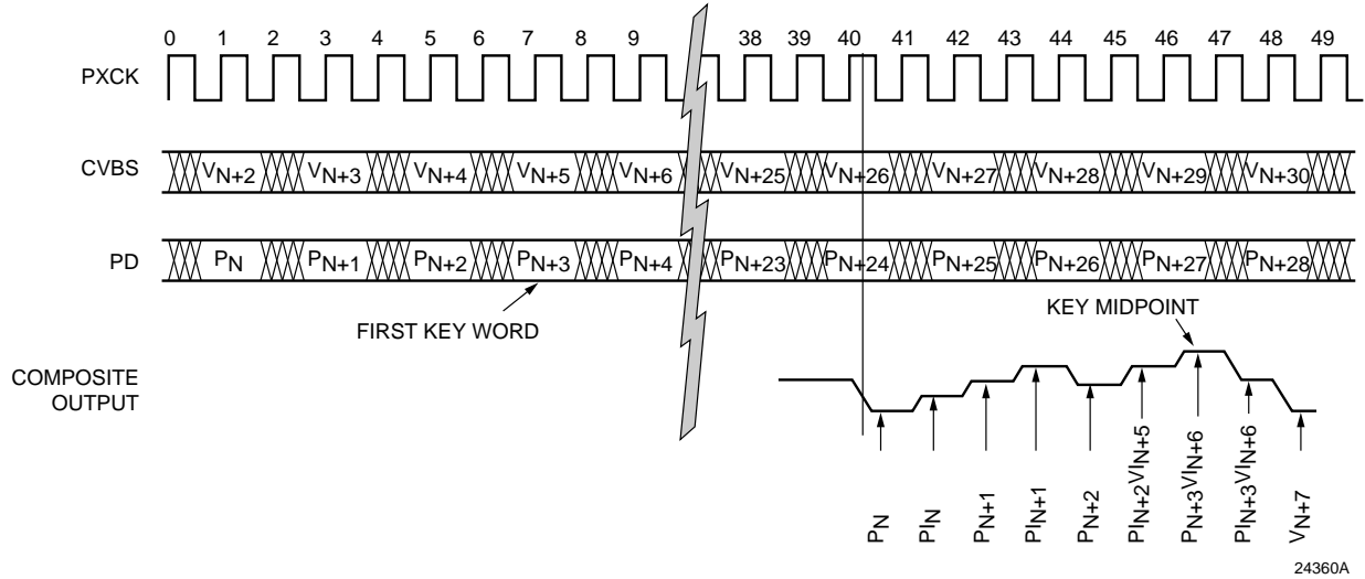
Figure 23. Data Keying
