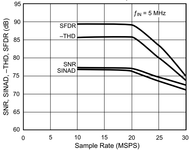
Performance Versus Sample Rate
