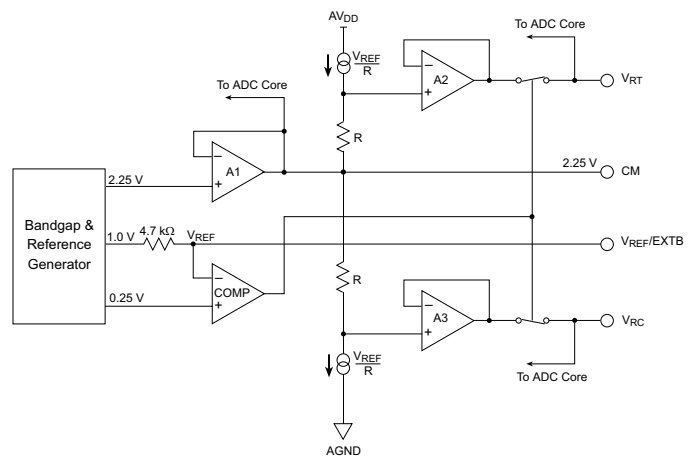
Figure 2 – Equivalent Reference Circuit
